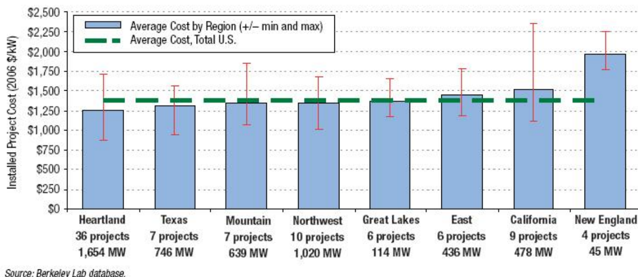
Figure E.1: Regional Installed Wind Project Costs
