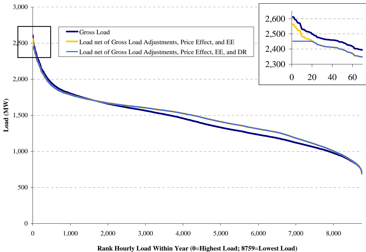
Figure G.28: 2011 SW-CT Net Load with Gross Load Adjustments, Fuel Price Effect, and Reference DSM in Low Stress Scenario
