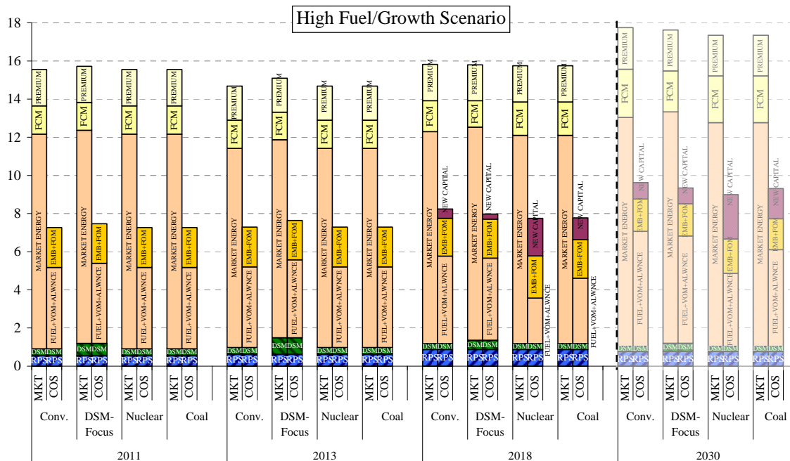
Figure 3.8: Average Customer Cost Components (¢/kWh)
