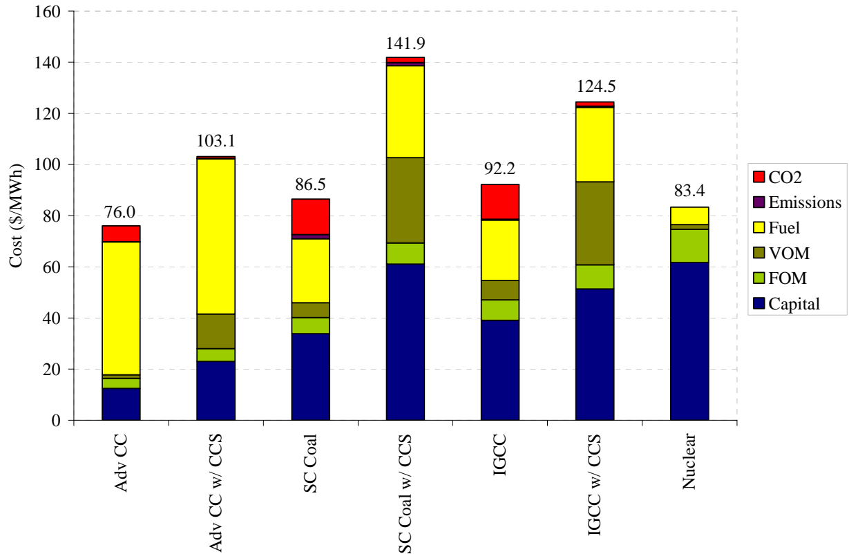
Figure C.1: Levelized Electricity Cost for Baseload Technologies (Current Trends parameters)
