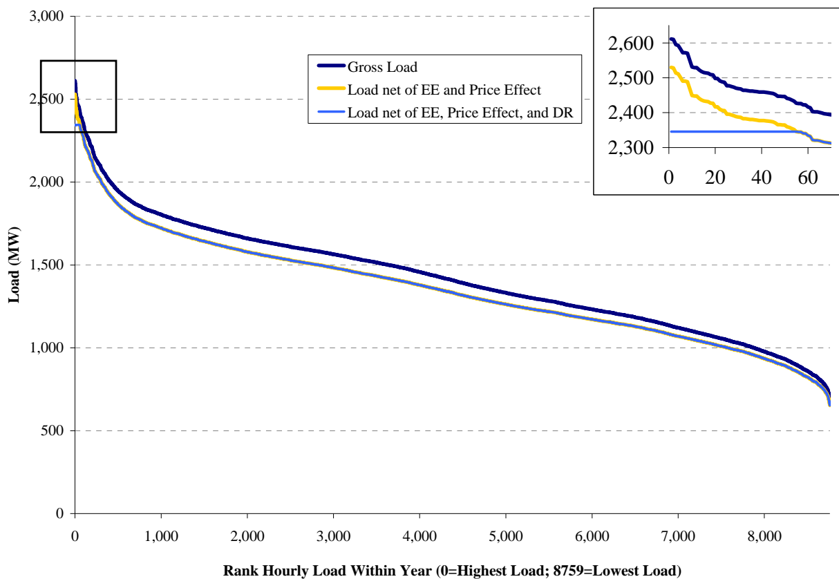
Figure G.24: Net Load with Fuel Price Effect and Reference DSM in the Strict Climate Scenario: 2011 SW-CT Example
