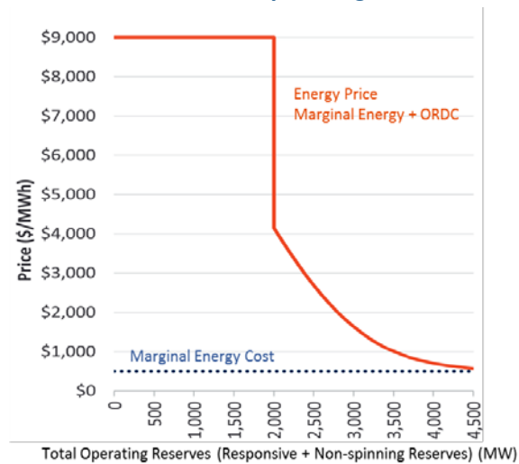
Figure 3: Illustration of ERCOT Operating Reserve Demand Curve
