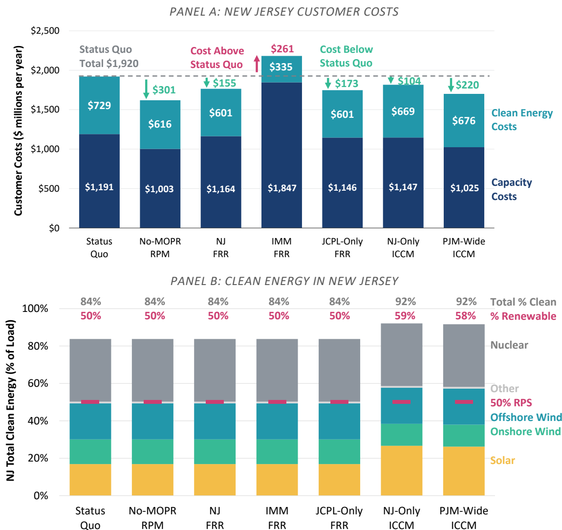
FIGURE 1: NEW JERSEY CUSTOMER COSTS AND SUPPLY MIX IN 2030 BY RESOURCE ADEQUACY DESIGN
