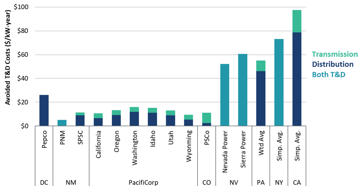
FIGURE 3: BRATTLE SURVEY OF AVOIDED T&D COSTS
