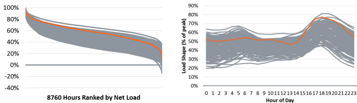
FIGURE 2: NET LOAD DURATION CURVES AND HOURLY LOAD SHAPES
